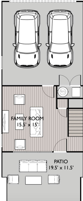
FIRST FLOOR PLAN - 320 SF
